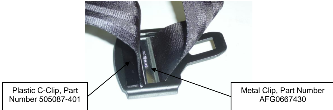
Figure 1: Correct assembly of the Slider Assembly Part Number 504802-403-142
