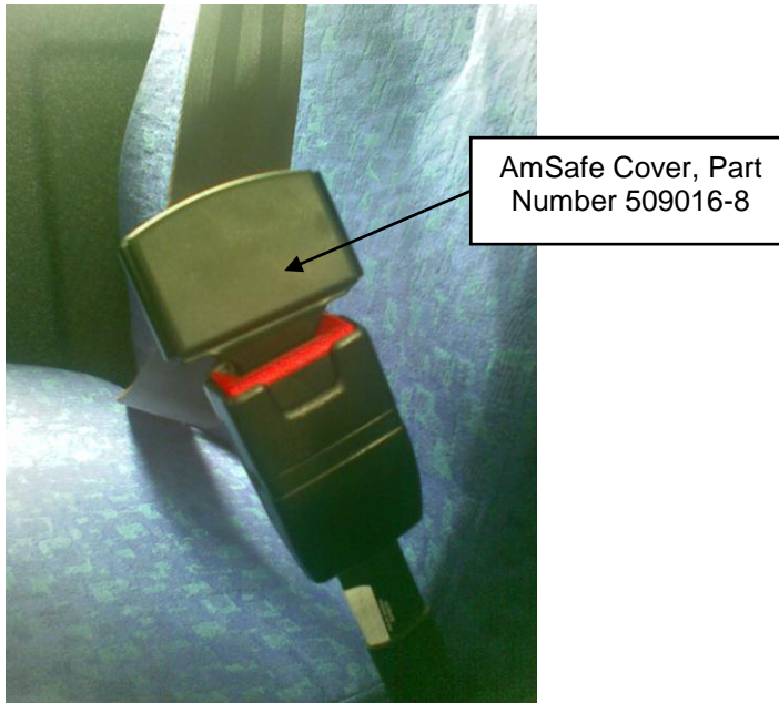
Figure 3: Harness with cover fitted
