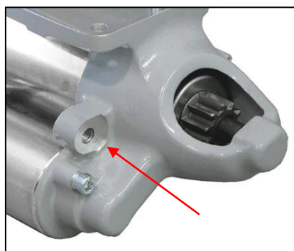
Figure 1 – Alternator Brace Mount Point
