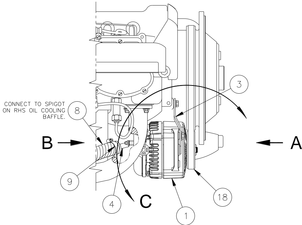
Figure 3 – Alternator Installation
