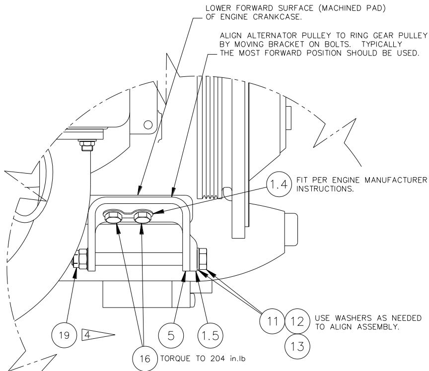
Figure 5 – Alternator Detail View B
