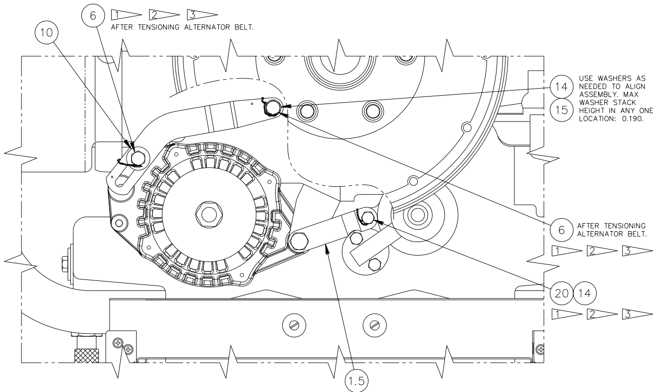
DETAIL VIEW A VIEW LOOKING AFT AT ALTERNATOR INSTALLATION
