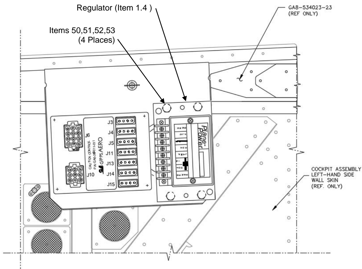
Figure 8 – Regulator Installation
